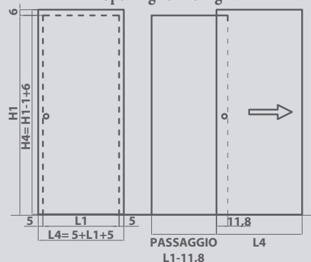
Apertura a destra opening to the right
